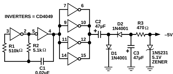
Figure 36. Generating a -5\text{ V} Supply When Only +12\text{ V} or +15\text{ V} Are Available
